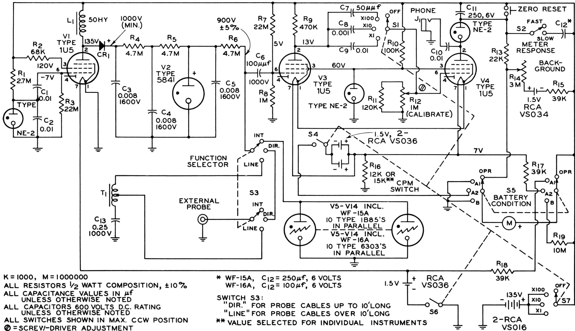
RCA Victor WF-15A, WF-16A
