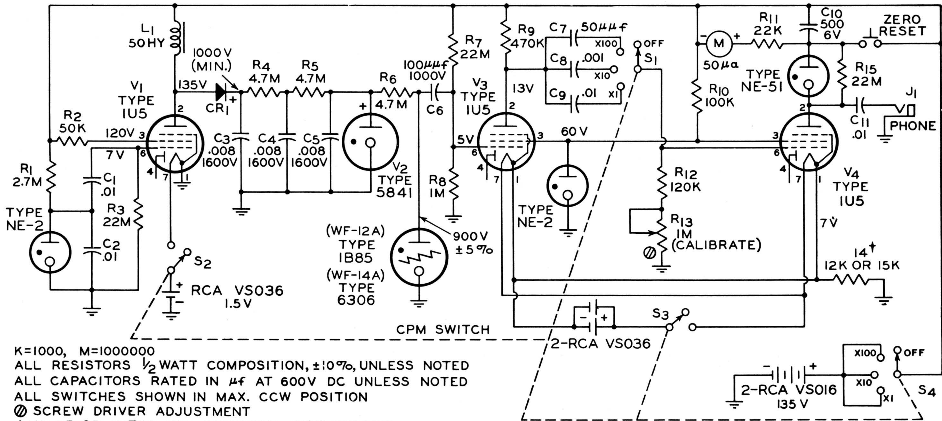
RCA VICTOR MODEL WF-12A, WF-14A
